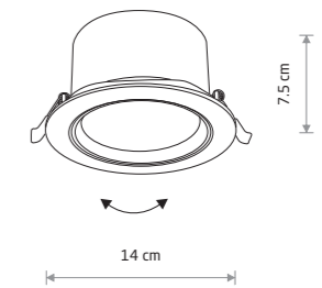
EGINA LED 15W
