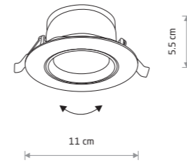
EGINA LED 10W
