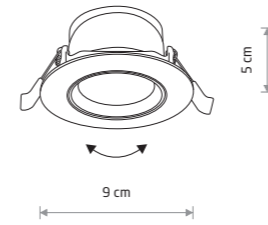
EGINA LED 5W
